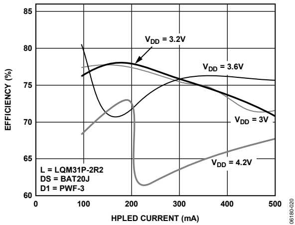
Figure 13. Efficiency P LED /P IN , One High Power White LED
