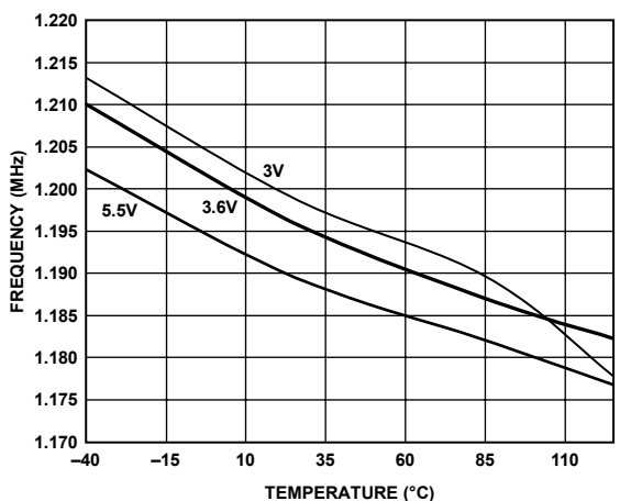
Figure 22. Oscillator Frequency vs. Temperature vs. V DD
