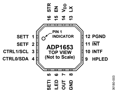
Figure 4. Pin Configuration
